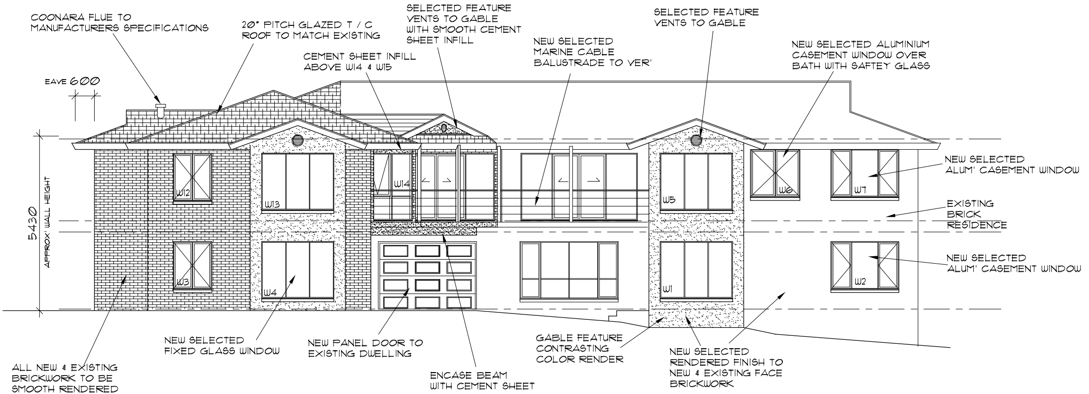
EAST FRONT ELEVATION " 1 " 1 : 100
