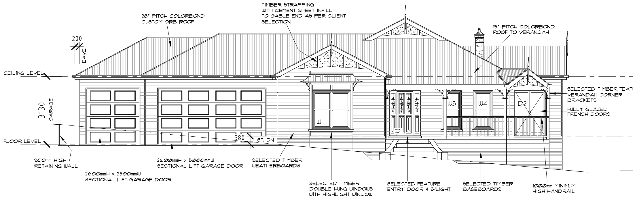
WEST FRONT ELEVATION "1" 1 : 100
