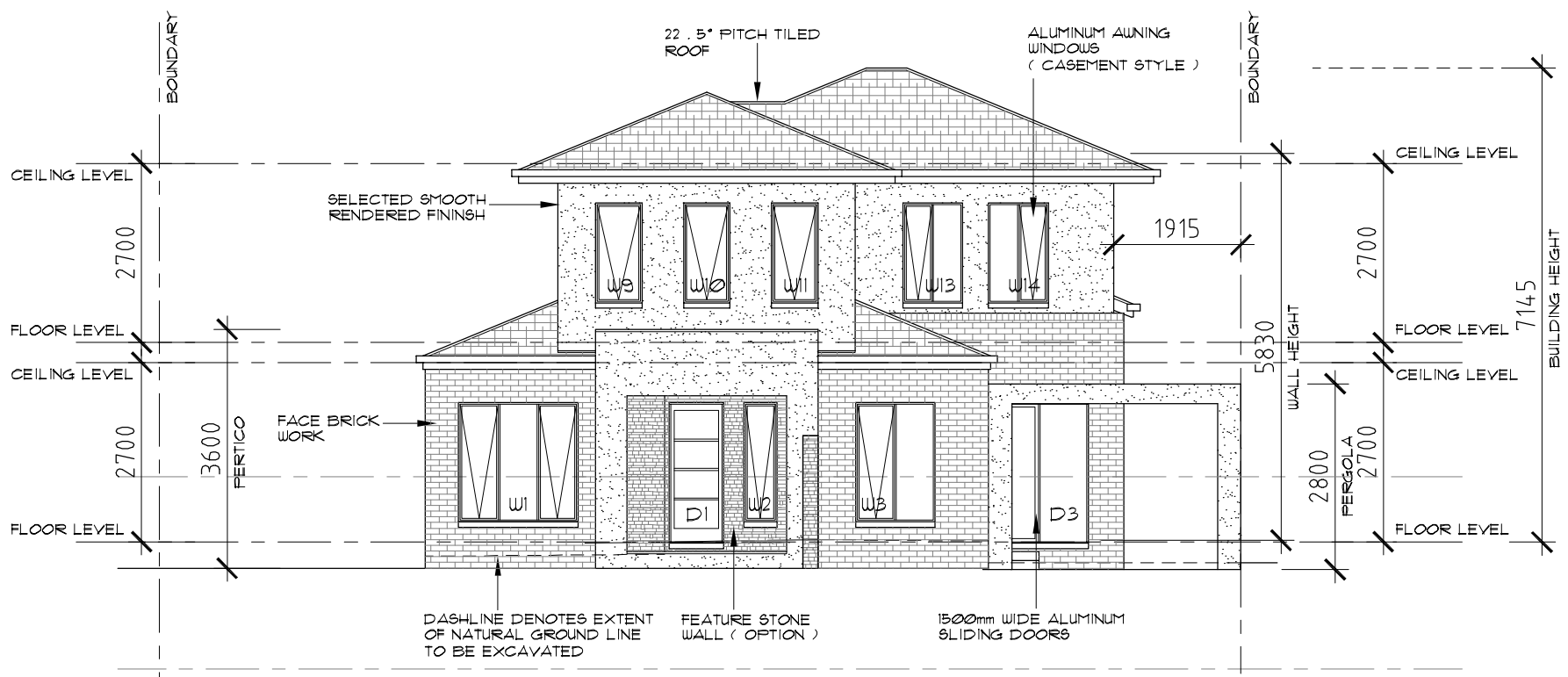
SOUTH FRONT ELEVATION " 1 " 1 : 100
