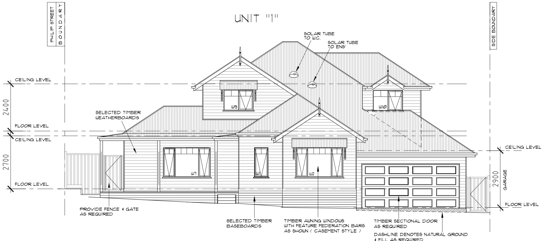
DAISY STREET SOUTH ELEVATION "2" 1:100
